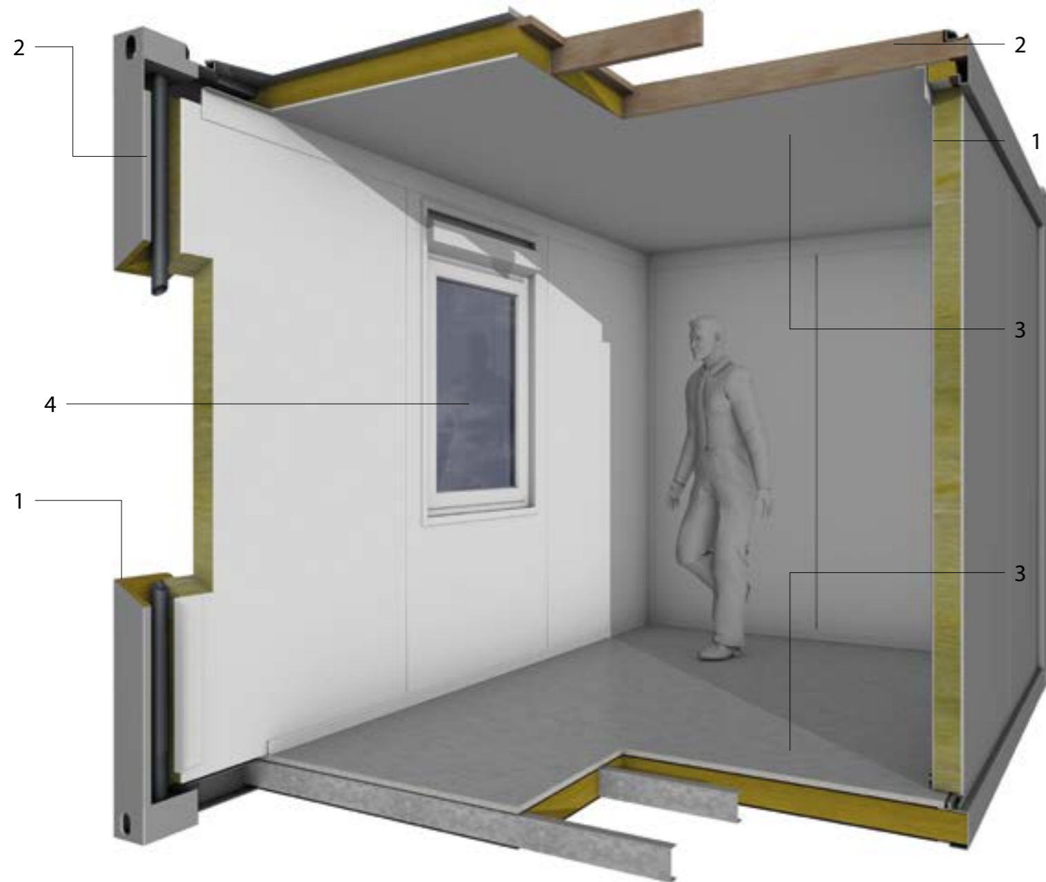
Standardised 20' modular space unit; exploded perspective
